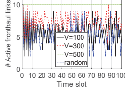
Fig. 4: Number of active fronthaul links vs. different time slots under RICH and random algorithms with V = 100, 300 and 500
