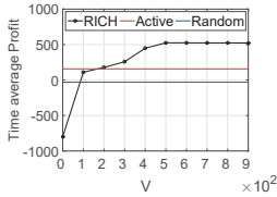
Fig. 2: Time average profit vs. different V under RICH , random and active algorithms
